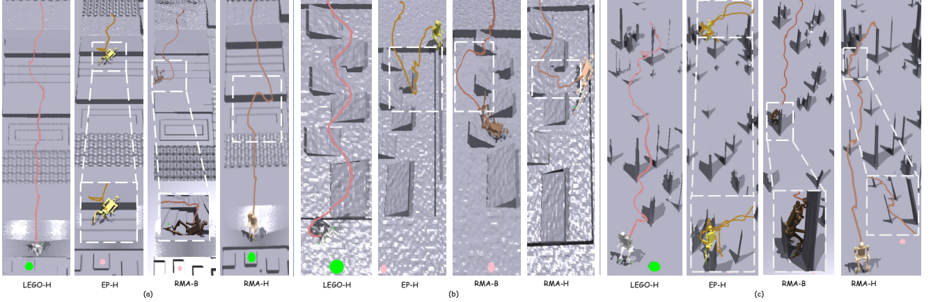
Figure 6. Qualitative comparisons between LEGO-H and other benchmarked methods. The trajectories, visualized through dynamically updated colored lines, depict the robots’ torso position as they traverse diverse trail environments. (a) illustrates the performance on a RandomMix trail featuring unobstructed views with varied terrain types. (b) highlights the results on a Ditch trail, where uneven terrain with slopes and gaps demands quick turns and agile leaps. (c) showcases the performance on a Forest trail, where extensive obstacles of different sizes and heights block the robot’s view. The zoom-in regions highlight the issues of the robots.
