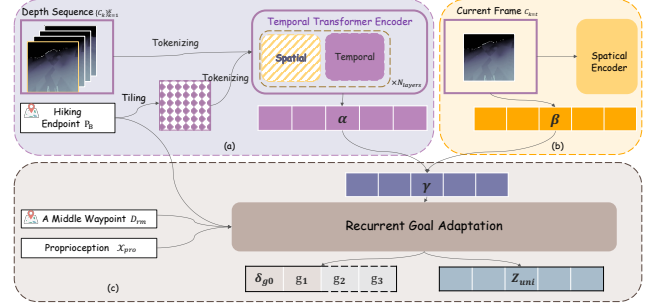
Figure 4. Architecture of TC-ViT. Three key components: (a) a goal-orientated temporal transformer encoder for robots cognizing surroundings with the final goal; (b) a dual process on the current depth frame for integrating spatially precise information to reflect the current state (c) a recurrent goal adaptation mechanism that integrates visual awareness, goal information, and proprioception.
