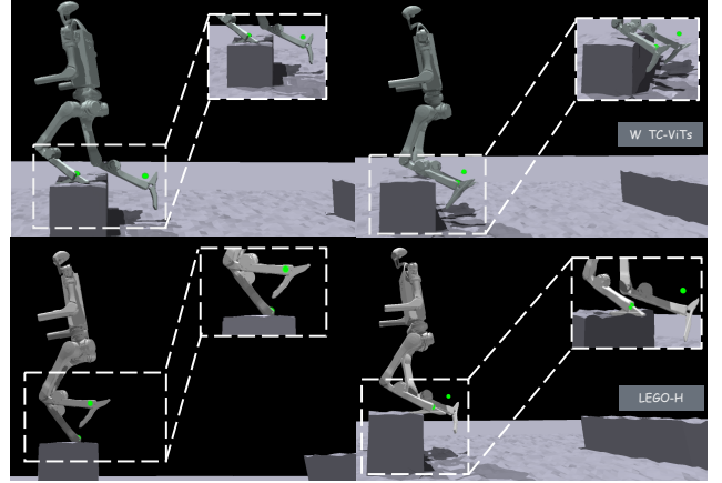
Figure 2. Qualitative ablation on with/without HLM. Snapshots from right to left depict two time steps of a robot traversing a hurdle obstacle. The top row illustrates behaviors without HLM, where unsafe movements lead to right leg collisions with the hurdle. The bottom row showcases behaviors with HLM, exhibiting coordinated and structurally rational actions that ensure stability and successful traversal with safe clearance.
